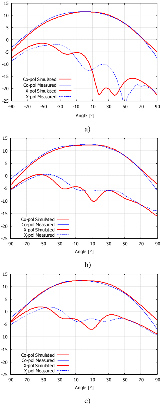
Figure 11: Comparison between the measured and simulated H-plane radiation patterns when the J3 array is fed at 2.62 GHz (a), 2.655GHz (b) and 2.69 GHz (c).
