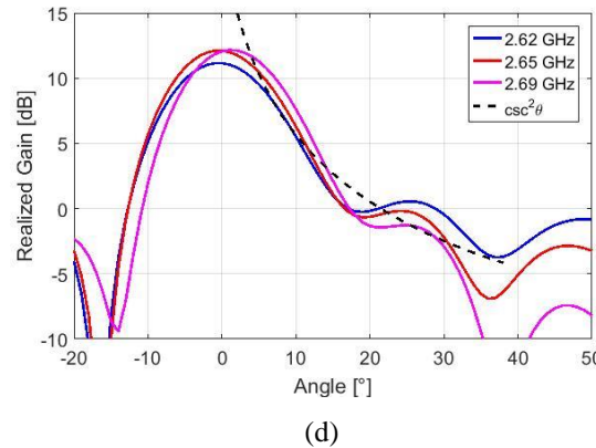
Figure 5: Results from the simulation of the array in Fig. 3 with periodic boundaries (spacing between columns equal to 65 mm). In (a) we have the reflection coefficient, in (b) the realized gain in the H-plane, in (c) the realized gain in the E-plane and in (d) a zoom on Fig. 5 (c) with the csc^2\theta pattern superposed for reference.
