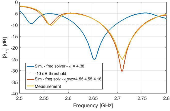
Figure 8: Reflection coefficient of the array in Fig. 3 simulated with CST using a \epsilon_r = 4.38 substrate in blue, using a (\epsilon_{rx}, \epsilon_{ry}, \epsilon_{rz}) = (4.55, 4.55, 4.16) substrate in red and the measured prototype first run in yellow.
