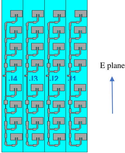
Figure 6: Front view of the 4-column array of microstrip rectangular patches with inset feeds. The array is fed from the center of each column via coaxial cables.
