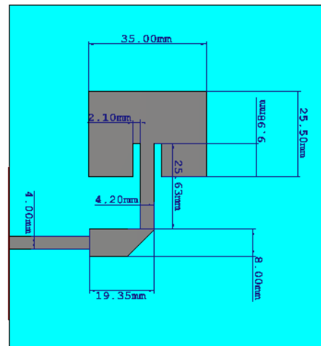
Figure 1: Front view of the optimized rectangular patch antenna with an inset feed, the feeding line arriving at the patch, a mitered bend and two quarter wavelength transformers.
