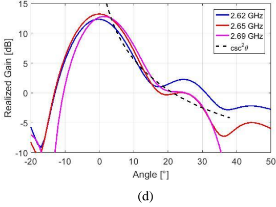
Figure 4: Results from the simulation of the array in Fig. 3. In (a) we have the reflection coefficient, in (b) the realized gain in the H-plane, in (c) the realized gain in the E-plane and in (d) a zoom on Fig. 4 (c) with the csc^2\theta pattern superposed for reference.
