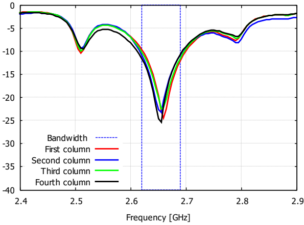
Figure 9: Reflection coefficient of one linear array among the three others.
