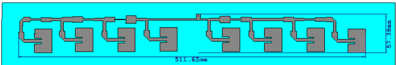
Figure 3: Front view of the optimized linear array of microstrip rectangular patches with inset feeds (Fig. 1). The array is fed from the center via a coaxial cable. Two microstrip lines of different lengths realize the phase difference between the four patches to the left and the four patches to the right.
